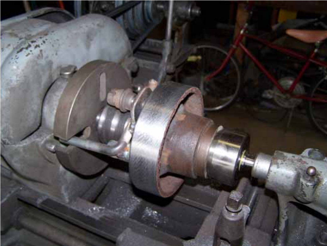
4. Turning down the front rotor to install Corvette rotors
